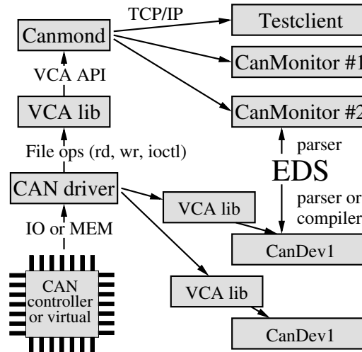
Figure 1-1. LinCAN architecture
