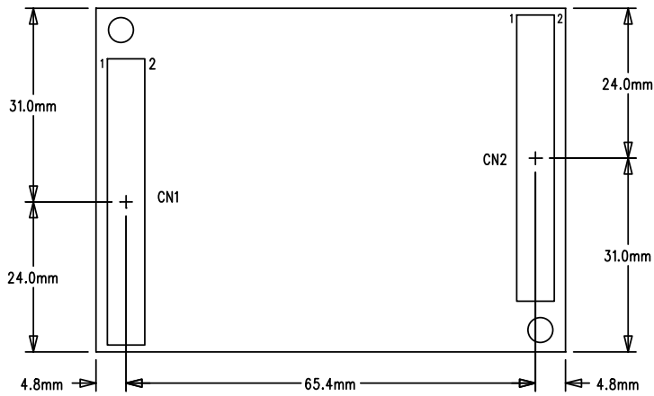
Connector Placement Top View
