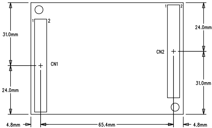
Connector Placement Top View
